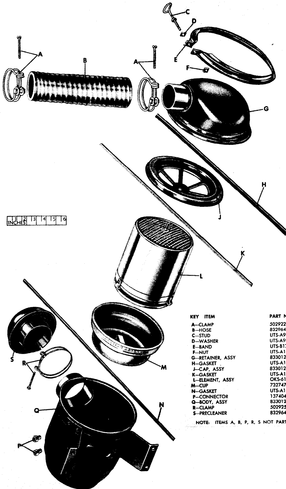
Figure 03-6. Air cleaner, assy (8329642)—exploded view
