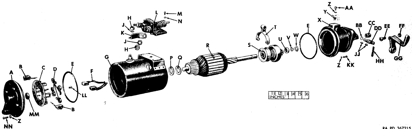
Figure 06-4. Starter, assy (8328132) Auto-Lite, 24-volt—exploded view
