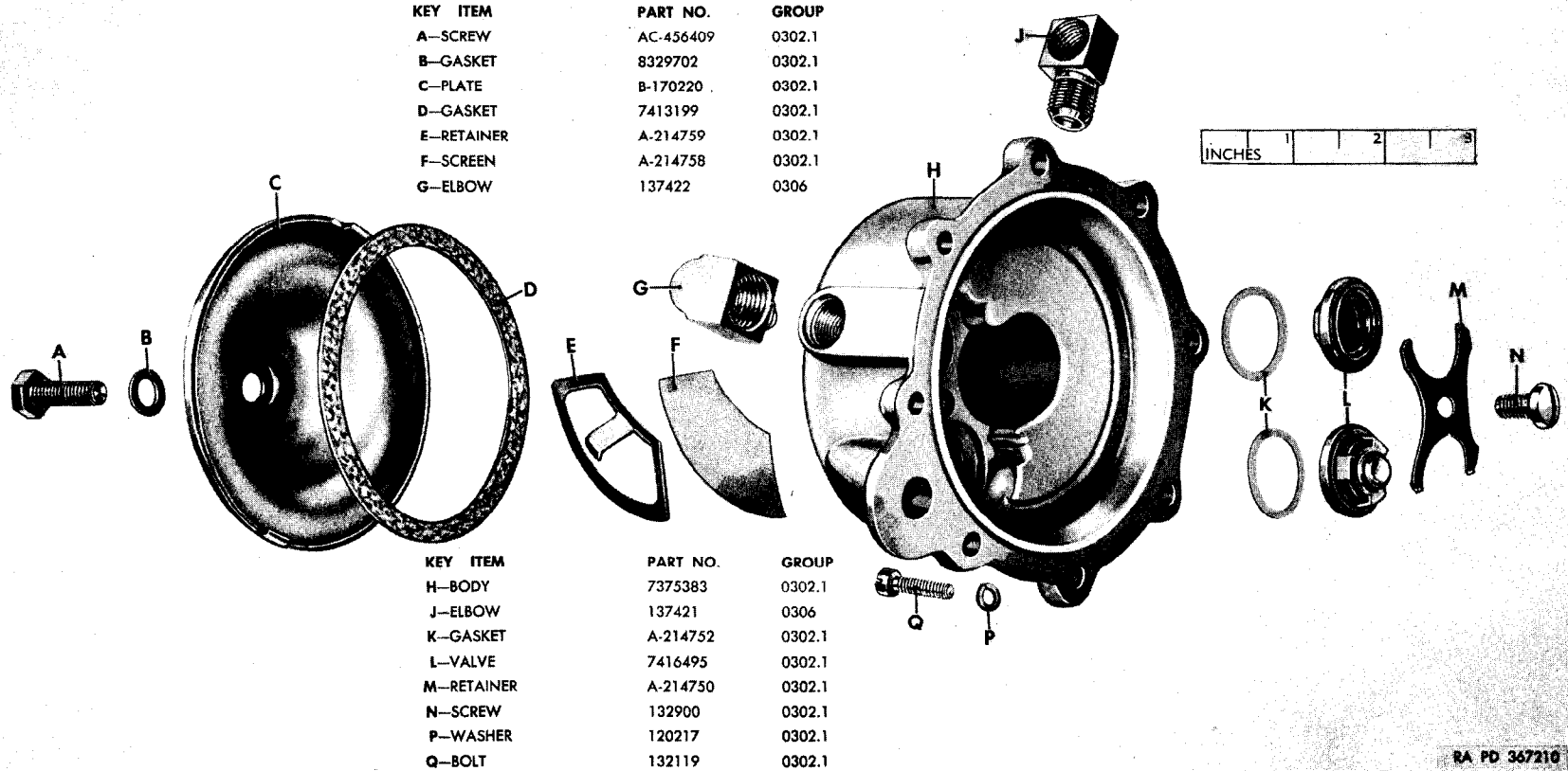
Figure 03-5. Fuel and vacuum pump (vacuum section)—exploded view
